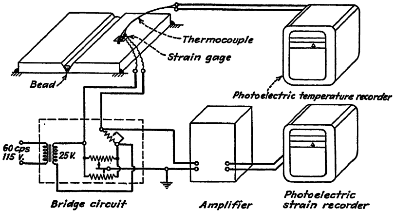
Strain gage setup for studying strains associated with welding.
